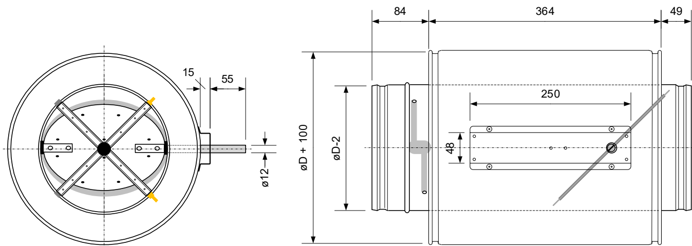
Type VSR-DW (double wall construction), drawn model 200
