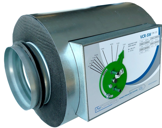
Type VCR-DW
