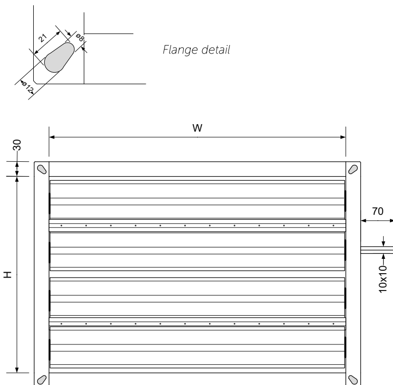
Type VSQ-SW (single wall construction), drawn model 600x400
